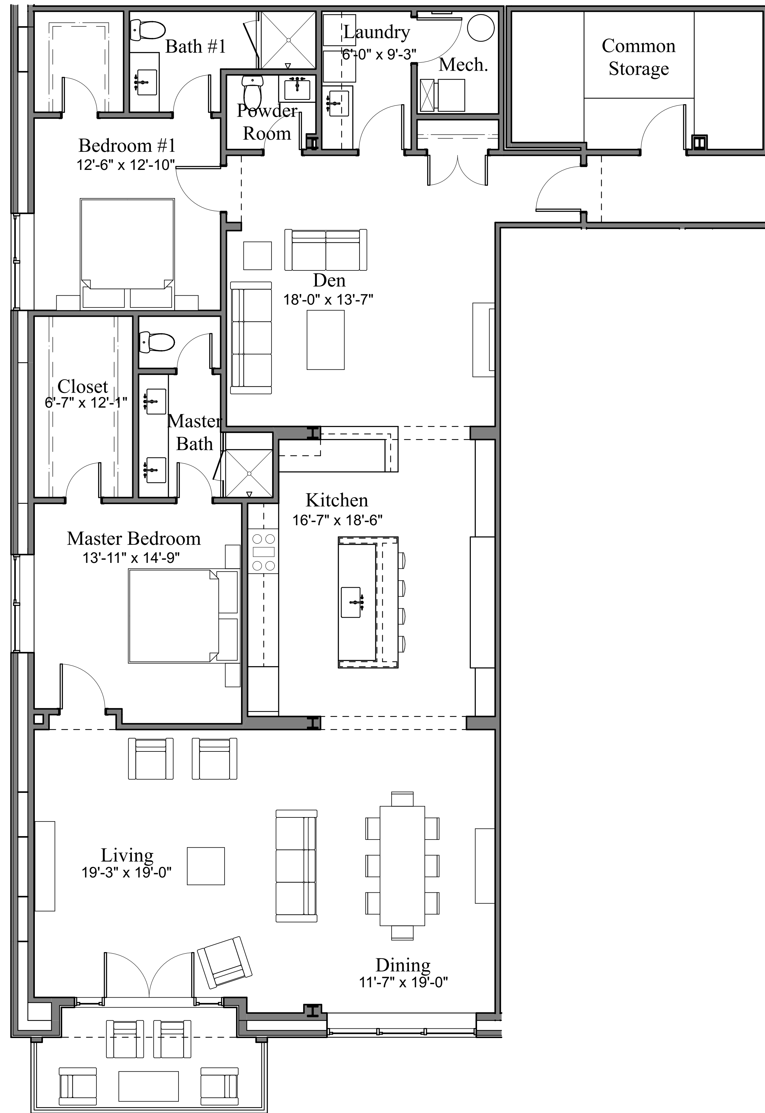
Units 103, 203 & 303 Option A
